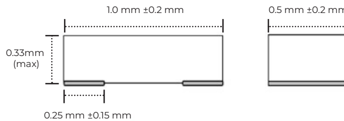
Figure 6: The LSCND1005CCTR47MH external dimensions (units: mm).
