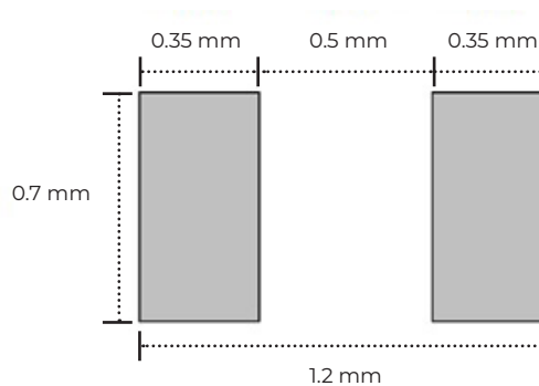
Figure 7: The LSCND1005CCTR47MH recommended land pattern (units: mm).
