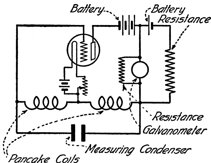
How the various instruments used in the ultra-micrometer are connected.
