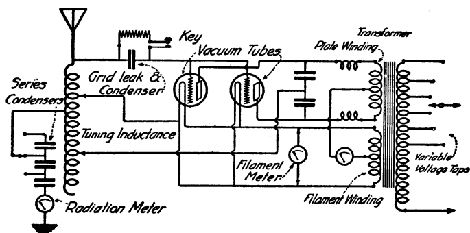
Transmitter No. 4. A ten-watt combination telegraph transmitter.
