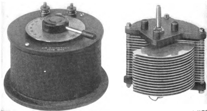
The type of variable condenser used in radio receiving circuits
