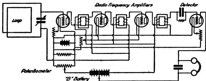
Connections for a radio-frequency amplifier using the loop or indoor antenna. This is receiving outfit No. 8.
