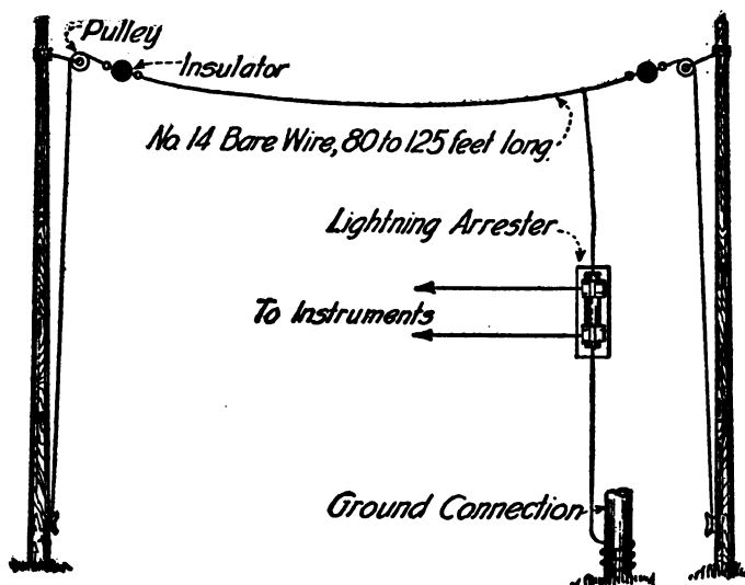
Constructional details of a simple one-wire aerial.
