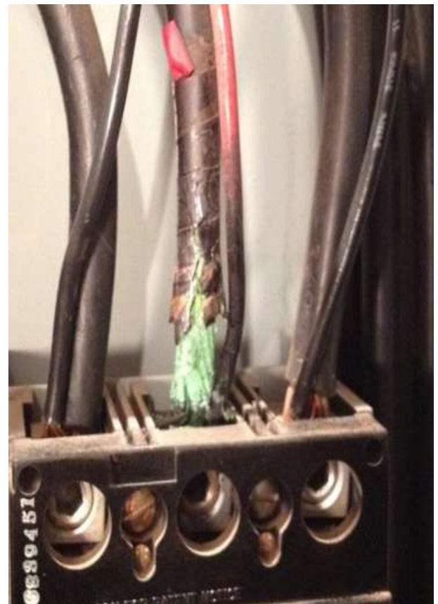
Above Fig. 12: Duct or gaffer’s tape works just fine for identifying AC disconnects.
