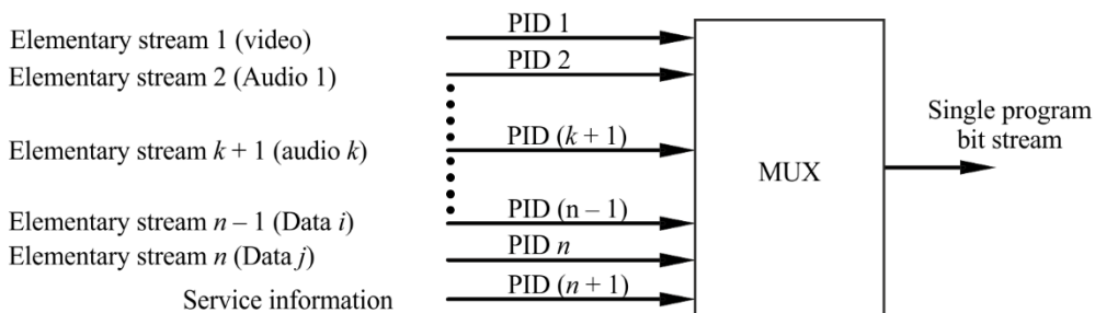
FIGURE 9.5 Illustration of multiplexing to form a single program stream
