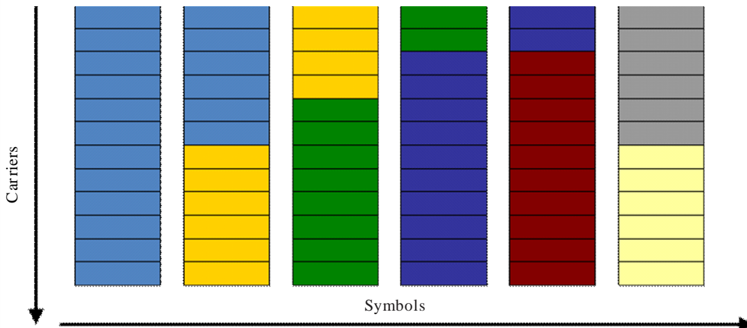
FIGURE 9.7 DVB-T2 system concept of fully transparent physical-layer pipes
