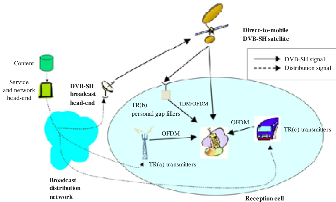
FIGURE 9.33 General view of a typical implementation of DVB-SH
