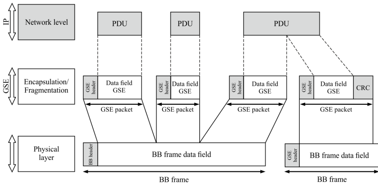
GSE encapsulation within DVB protocol stacks
