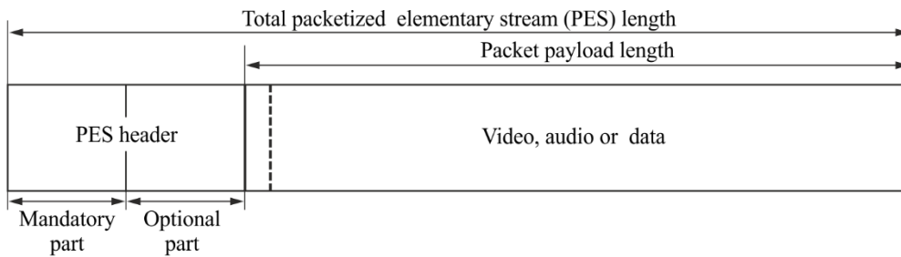
FIGURE 9.4 PES-packet structure
