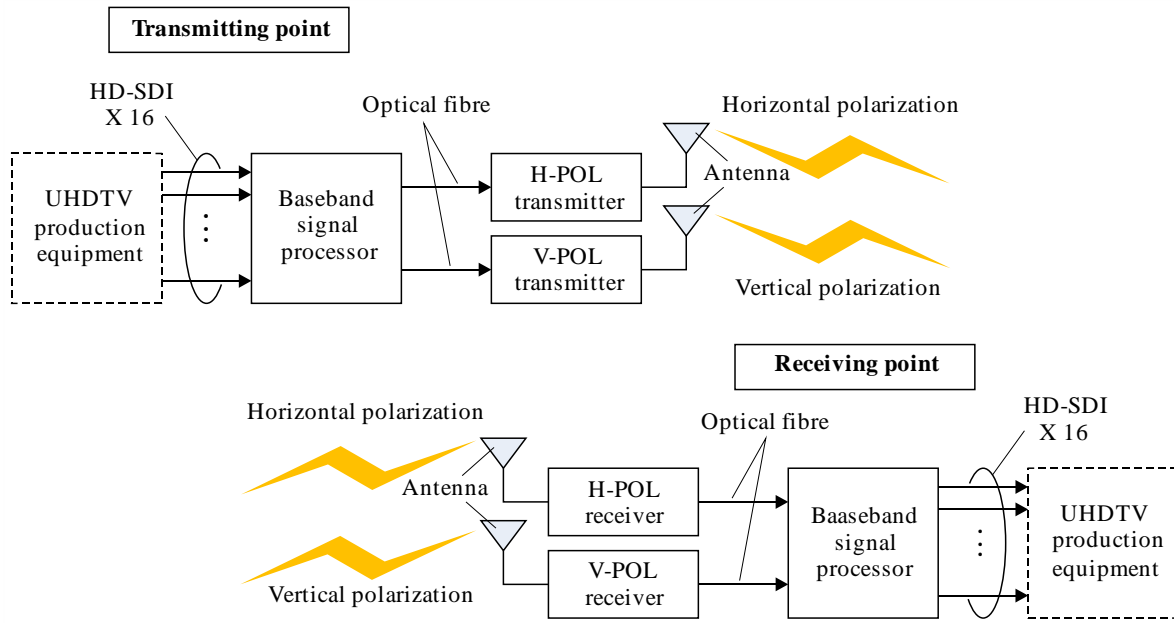
FIGURE 15.6 Overview of the temporary 120 GHz band video link for 8K
