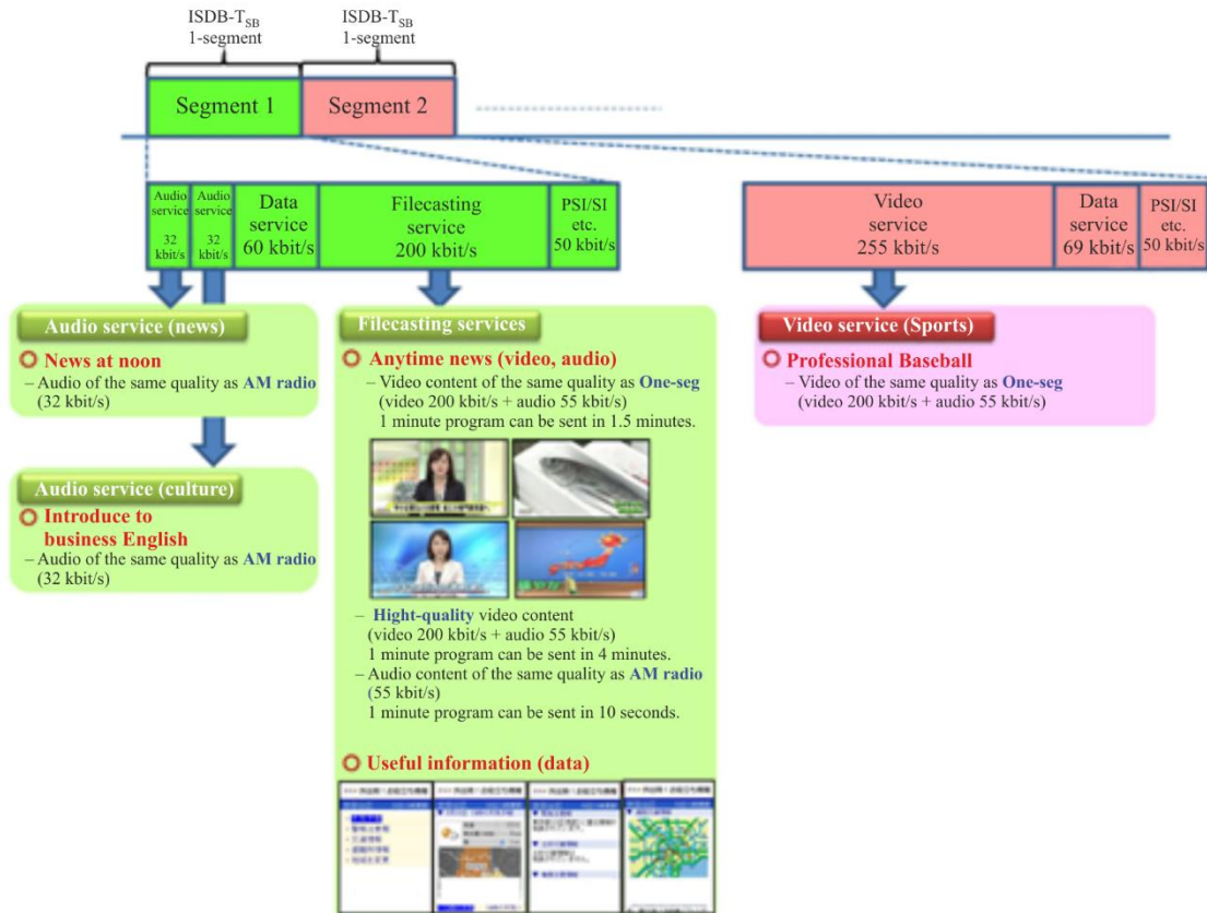
Example of 1-segment service
