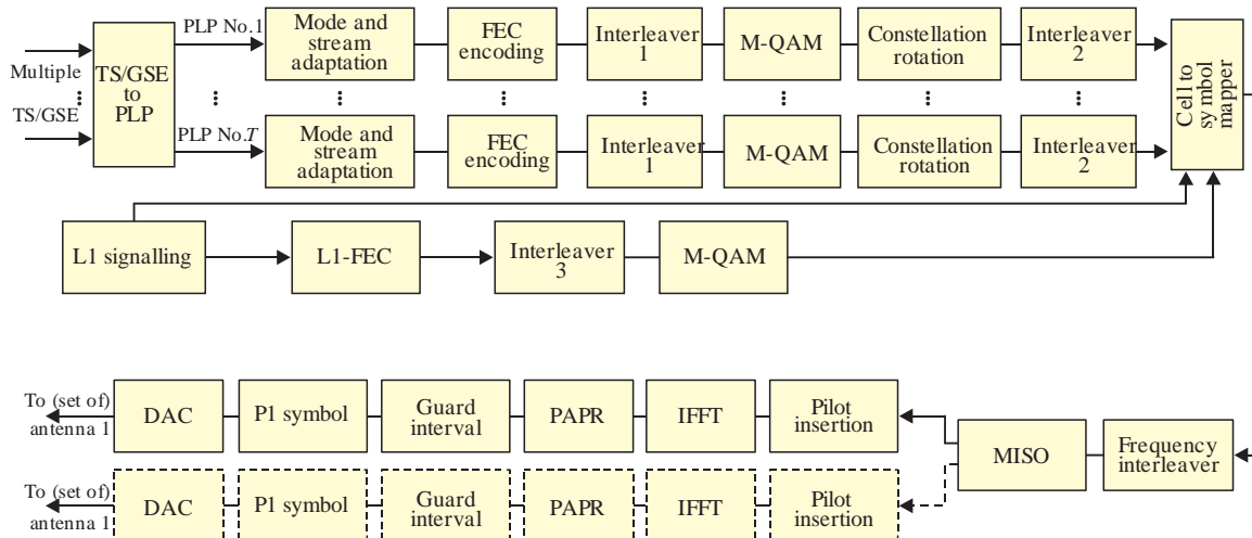
DVB-T2 block diagram
