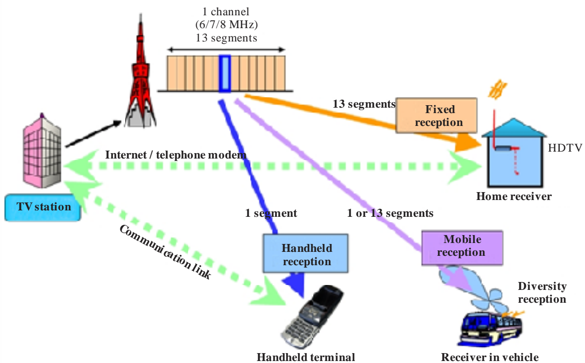
FIGURE 9.42 ISDB-T Service
