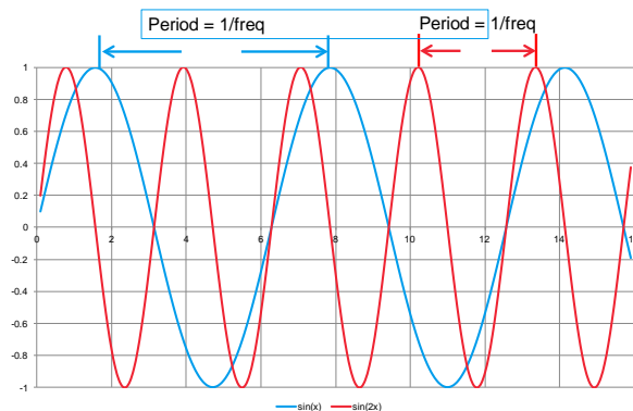
Figure 2. Basic sine waves are used to carry information by varying their frequency, amplitude, and/or phase.
